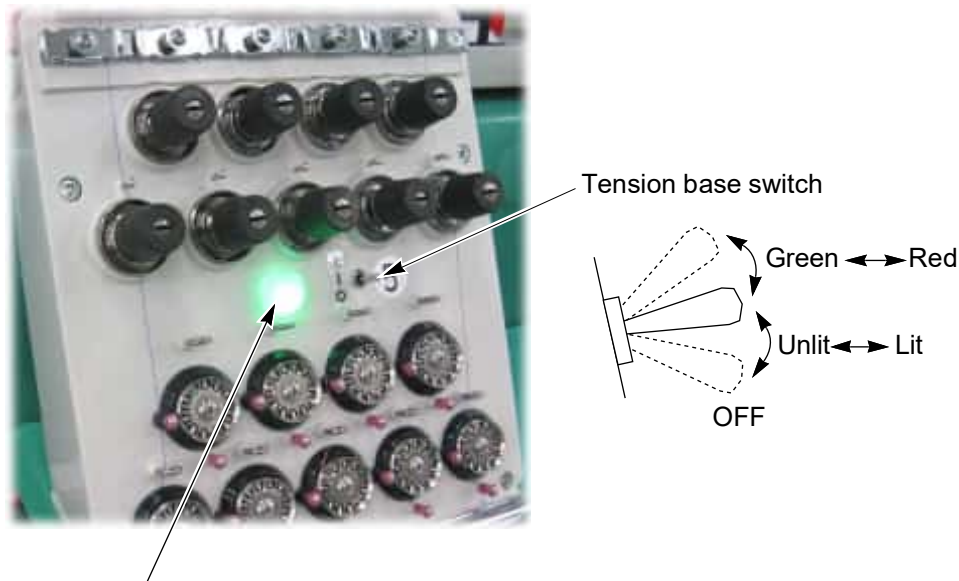
Thread breakage indicator lamp
